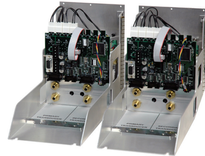
Channel module
